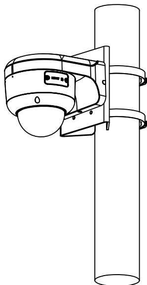
Pole Mount(Vertical)
