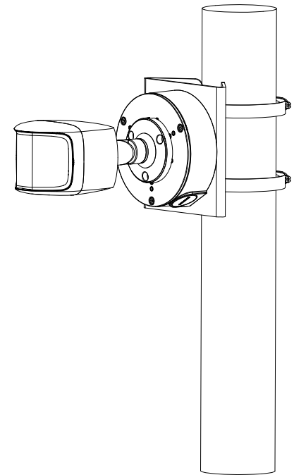
Pole Mount(Vertical)
