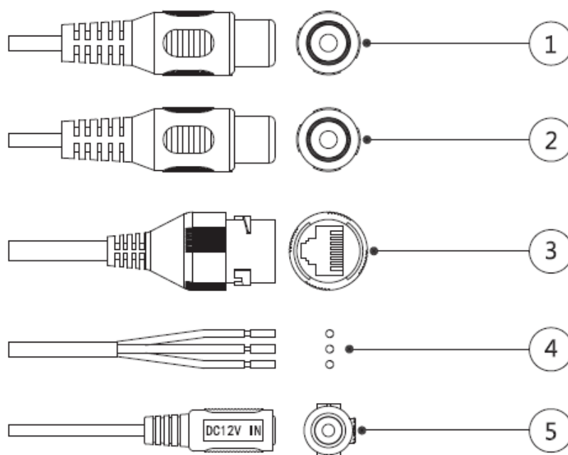
Figure 1-1 Cable list
