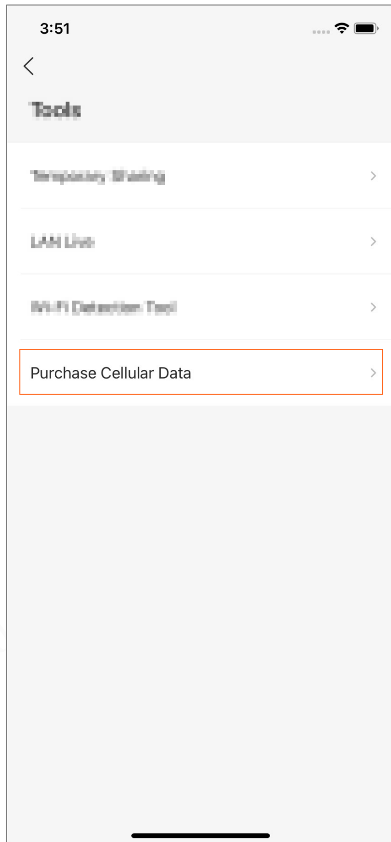
Figure 1-5 Tools page
