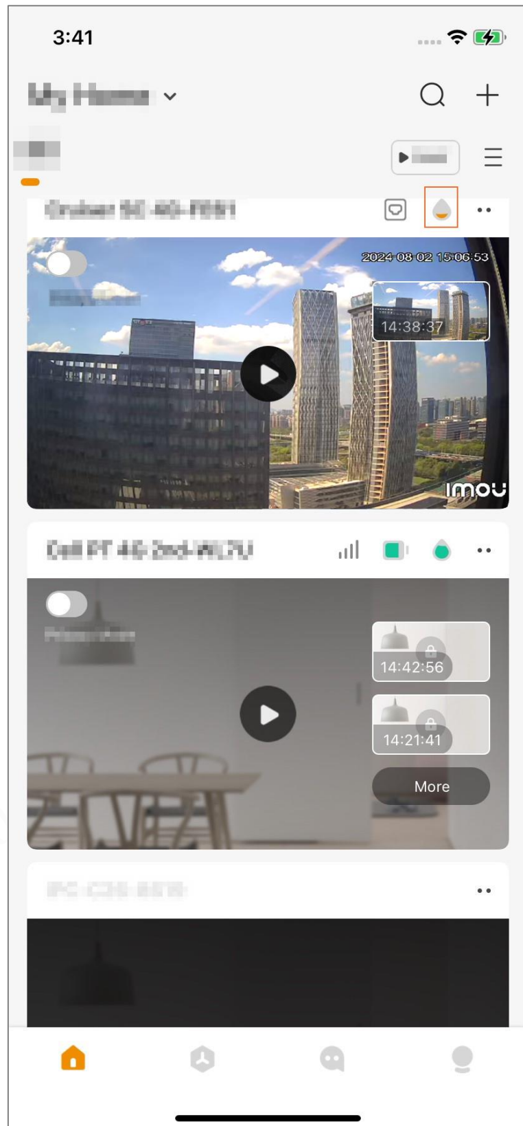
Figure 1-1 Home page
