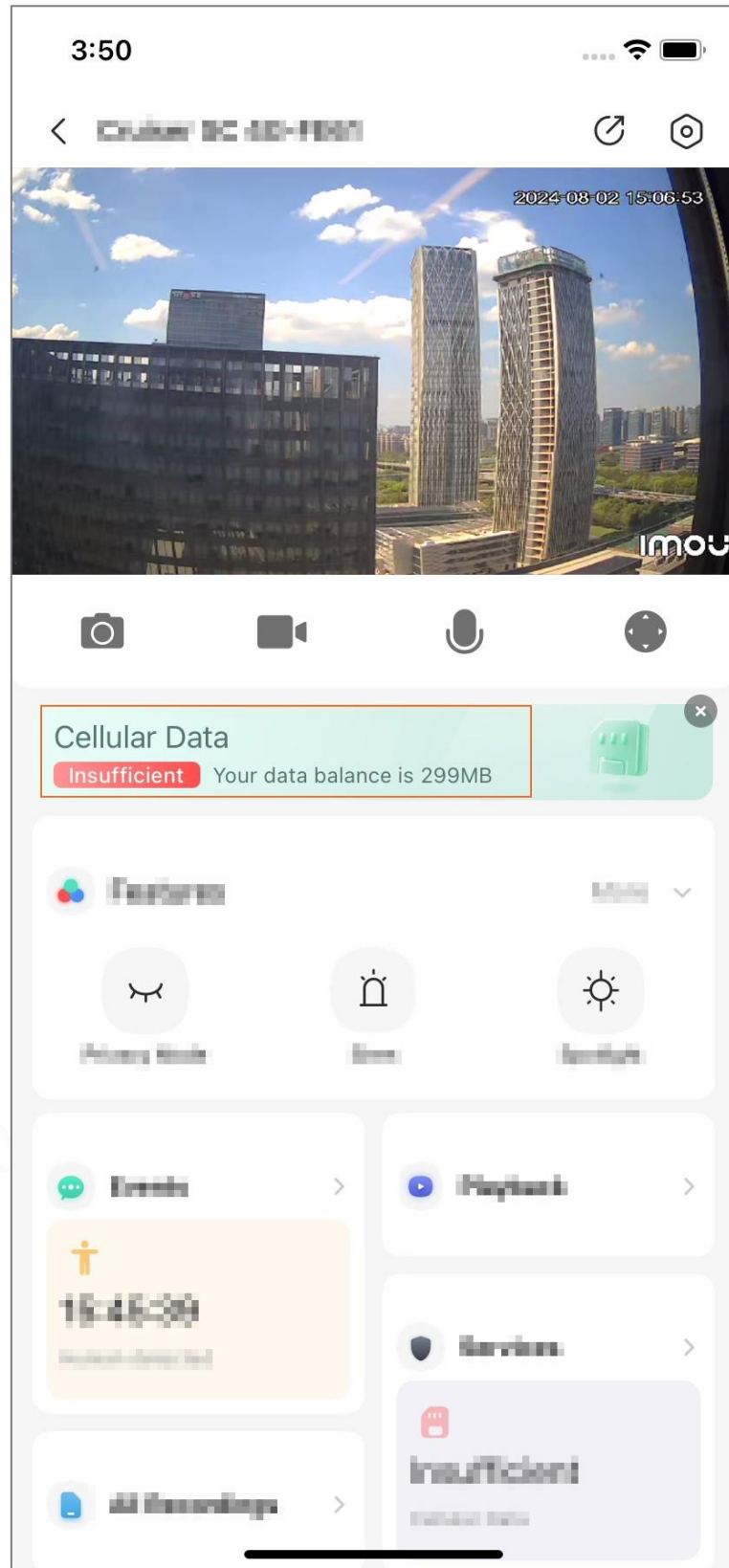
Figure 1-2 Preview page
