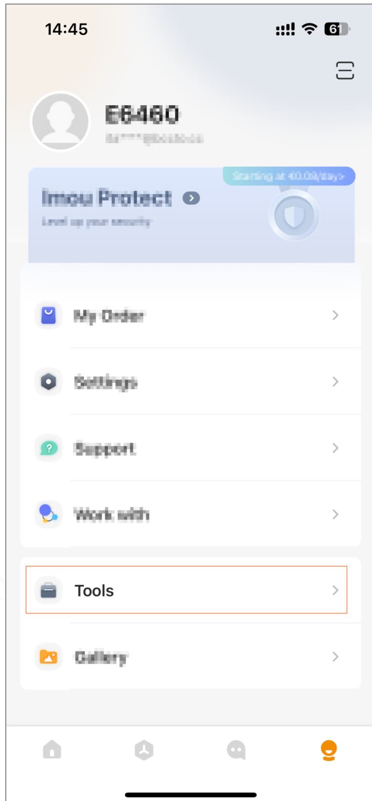
Figure 1-4 Me page
